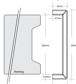
Cross Section. 1
